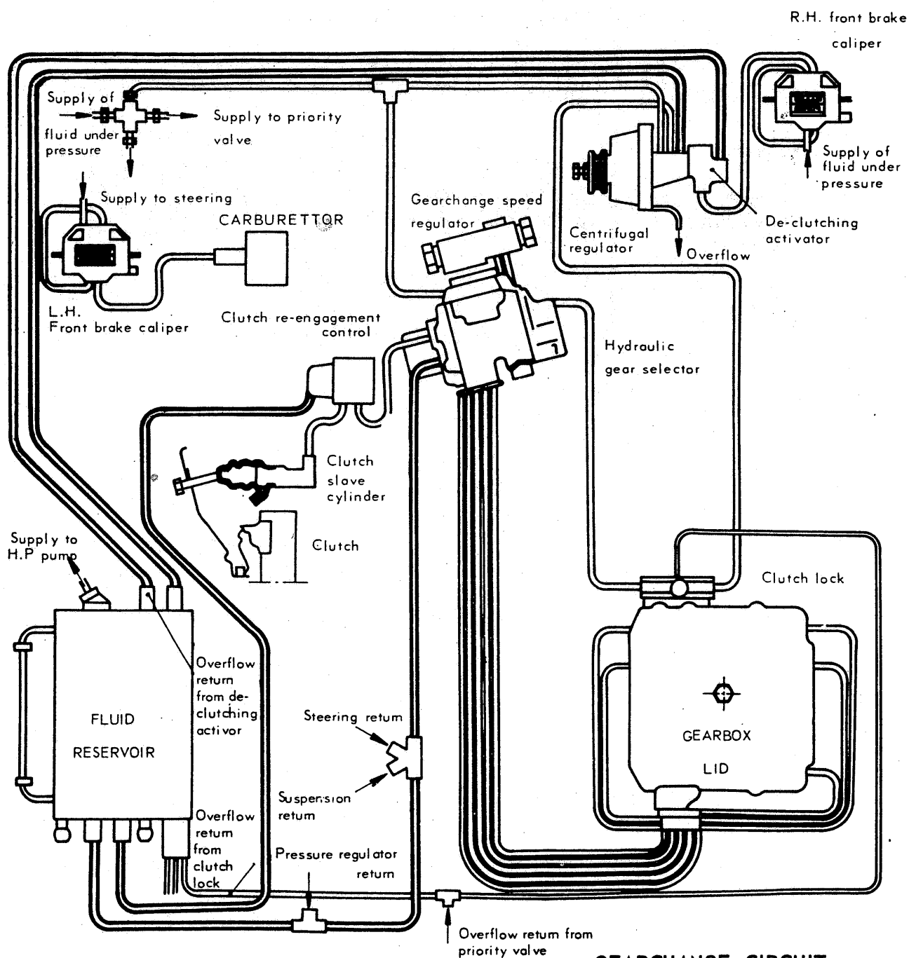
GEARCHANGE CIRCUIT
